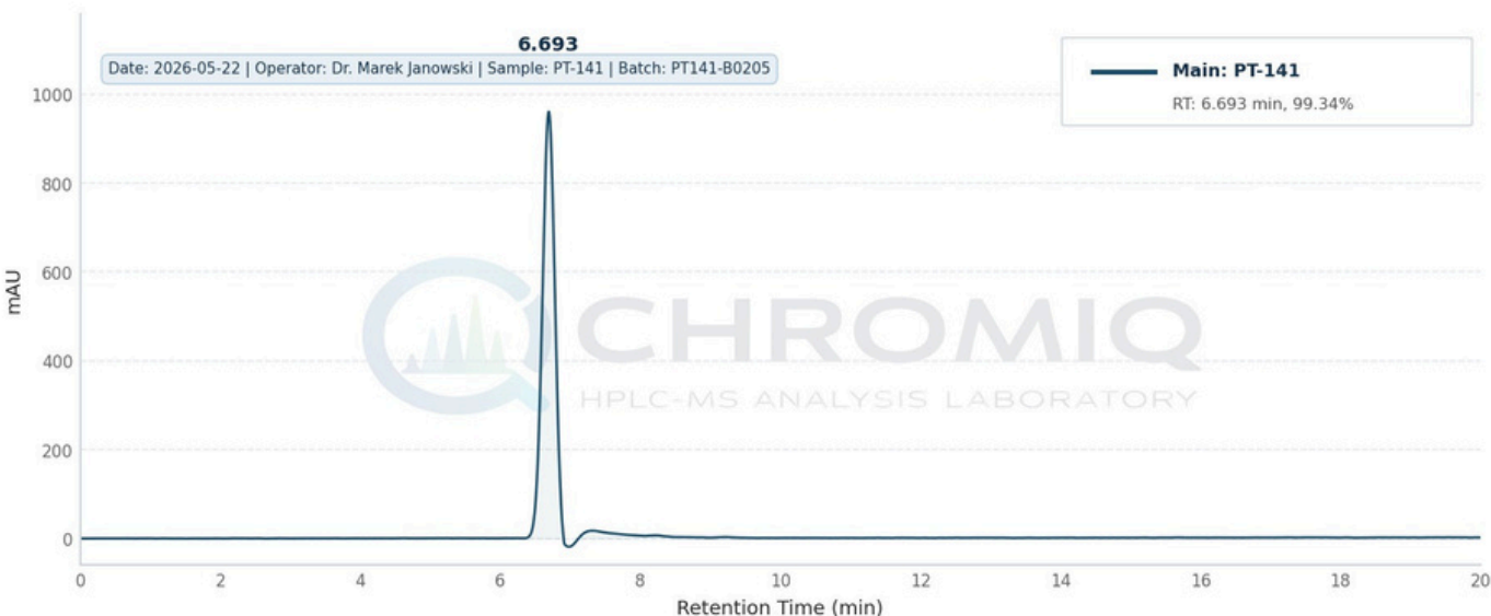
HPLC Chromatogram — PT-141, DAD1B @ 214 nm
